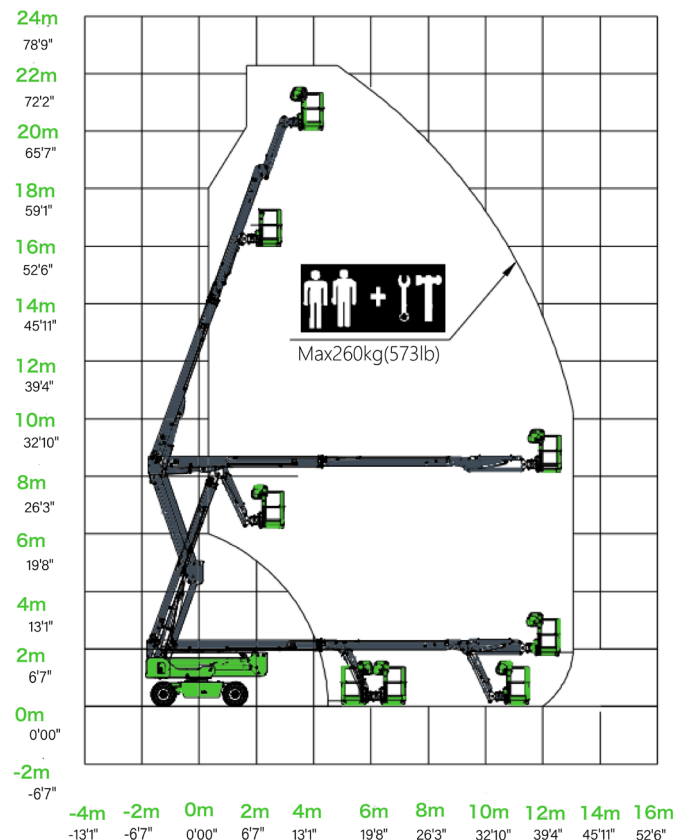
LA20JE Working Range
